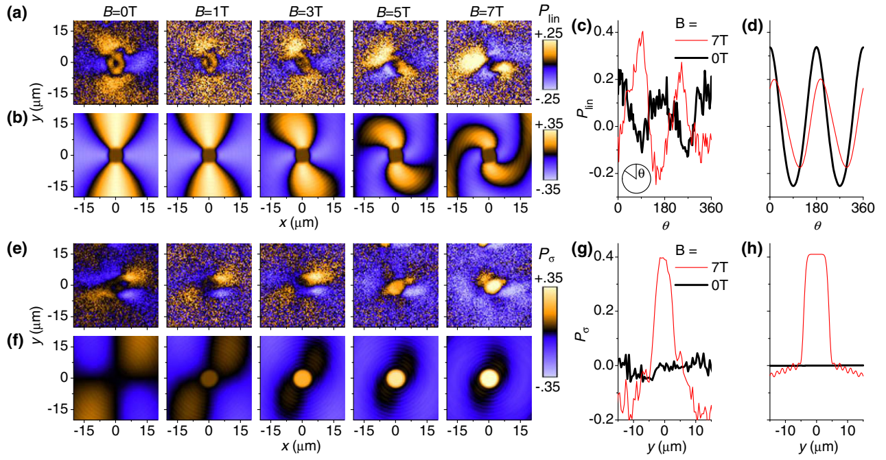
FIG. 2 (color online). Control of polarization patterns. Measured (a) and simulated (b) patterns of linear polarization of the emission of indirect excitons P_{\text{lin}} in the region of LBS for different magnetic fields perpendicular to the QW plane B . Measured (c) and simulated (d) azimuthal variation of P_{\text{lin}} at a distance from the LBS center r = 9 \mu\text{m} for B = 0 (black) and 7 T (red). Angles are measured from the y axis. Measured (e) and simulated (f) patterns of circular polarization of the emission of indirect excitons P_{\sigma} in the region of LBS for different B . Measured (g) and simulated (h) cross sections of P_{\sigma} at x = 0 for B = 0 (black) and 7 T (red). For all data, T_{\text{bath}} = 0.1 \text{ K} ; the LBS is at (105,75) in Fig. 1(c). See the Supplemental Material [31].
